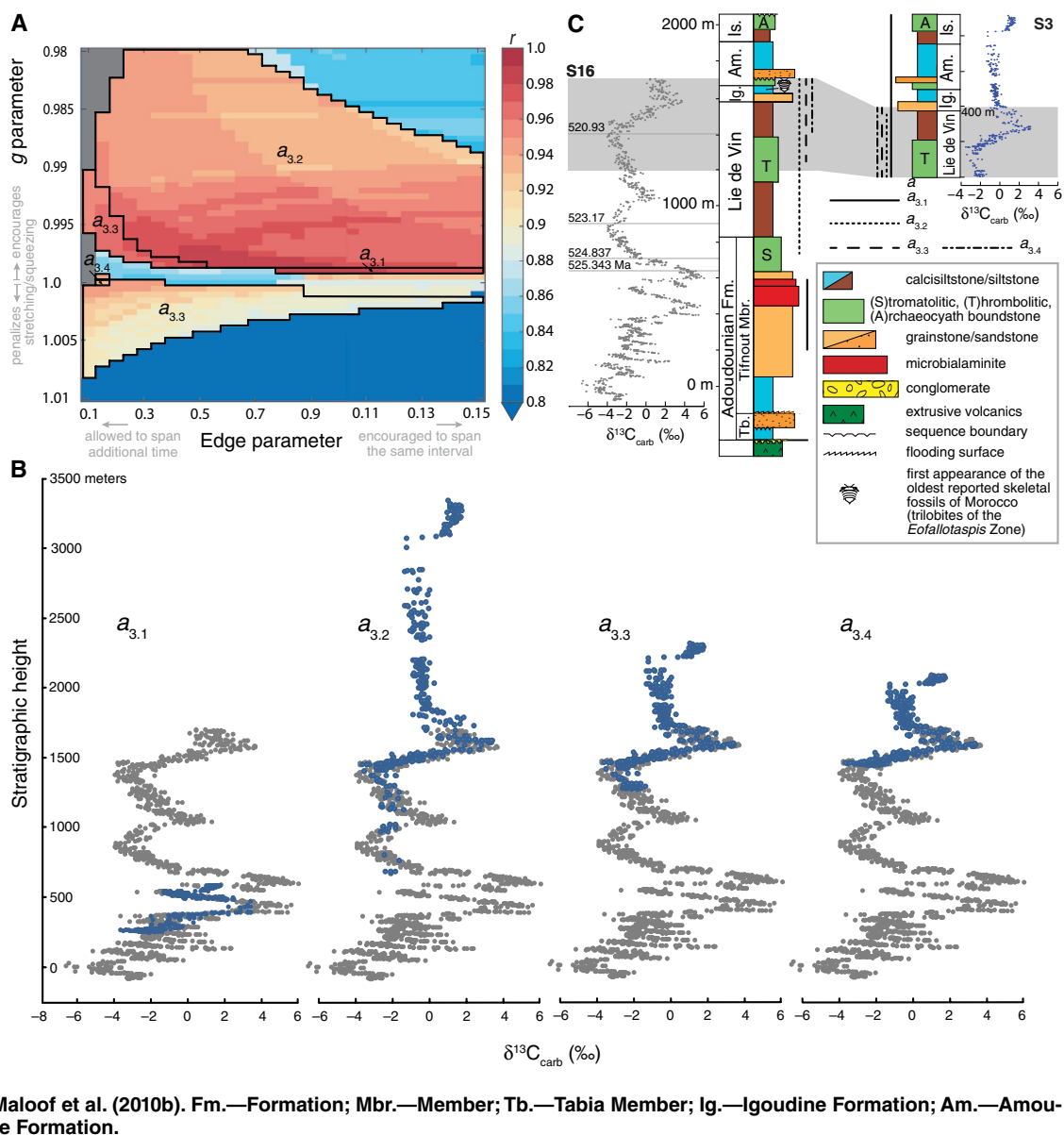
Figure 1. Optimal alignments of Cambrian Series 1–2 \delta^{13}\text{C}_{\text{carb}} (carb—carbonate) data from sections S3 (Talat N'Yissi) and S16 (Sidi M'Sal), Anti-Atlas, Morocco (Malooof et al., 2005, 2010b). A: Correlation coefficients ( 0.8 < r < 1 ) for solutions with specified pairings of g parameter (relating to the similarity of sediment accumulation rate at two stratigraphic sections during their shared interval of deposition) and edge parameter (relating to whether two sections span the same interval of time) (Sakoe and Chiba, 1978). Gray areas show parameter pairings that yield invalid alignments (<10% overlap). Solid black lines circumscribe parameter space for four distinct and significant alignment solutions ( a_{3,1} – a_{3,4} ). B: Alignments a_{3,1} – a_{3,4} , between S3 \delta^{13}\text{C} data (blue) and S16 \delta^{13}\text{C} data (gray), that correspond to parameter space in A. C: Lithostratigraphic correlation implied by alignments a_{3,1} – a_{3,4} . For example, solution a_{3,1} (solid line) correlates \delta^{13}\text{C}_{\text{carb}} data sampled from all S3 lithostratigraphic units to Adoudounian Formation at S16 (246–580 m). Shading covers visual correlation of Malooof et al. (2010a). Four radiometric dates shown on the S16 chronology are taken from Malooof et al. (2010b). Fm.—Formation; Mbr.—Member; Tb.—Tabia Member; Ig.—Igodine Formation; Am.—Amoulslek Formation; Is.—Issafene Formation.
