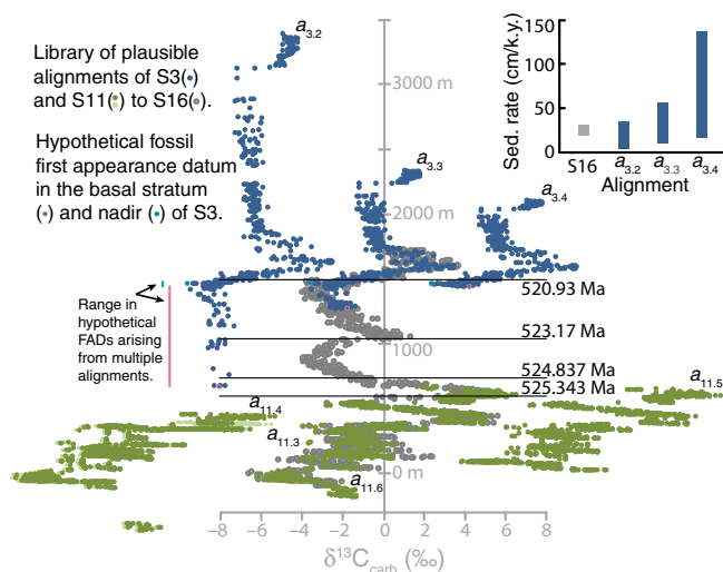
Figure 2. Dynamic programming-derived library of stratigraphically plausible, Cambrian Series 1–2 \delta^{13}\text{C}_{\text{carb}} (carb-carbonate) alignment solutions for sections S3 (Talat N' Yissi; blue circles; Maloof et al., 2005) and S11 (North Zawyat n' Bouzoul; green circles; Maloof et al., 2005) to section S16 (Sidi M'Sal; gray circles; Maloof et al., 2010b), Anti-Atlas, Morocco. Four radiometric dates shown on the S16 chronology are taken from Maloof et al. (2010b). Inset shows the range of sedimentation rates implied by alignment solutions a_{3,2} , a_{3,3} , and a_{3,4} (Fig. DR4 [see footnote 1]) compared to that for S16 (Maloof et al., 2010b). Alignment of S11 to S16 strata below the oldest radiometric constraint precludes the calculation of absolute sedimentation rates.
