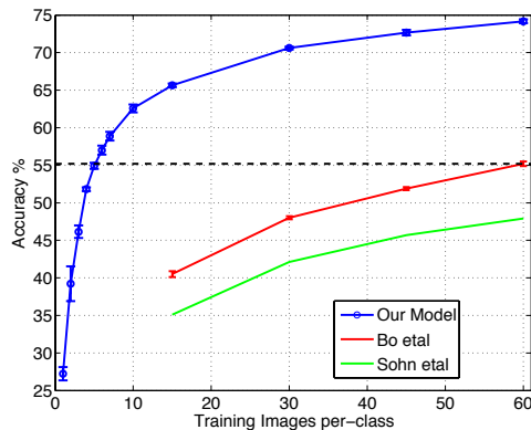
Figure 9. Caltech-256 classification performance as the number of training images per class is varied. Using only 6 training examples per class with our pre-trained feature extractor, we surpass best reported result by (Bo et al., 2013).
